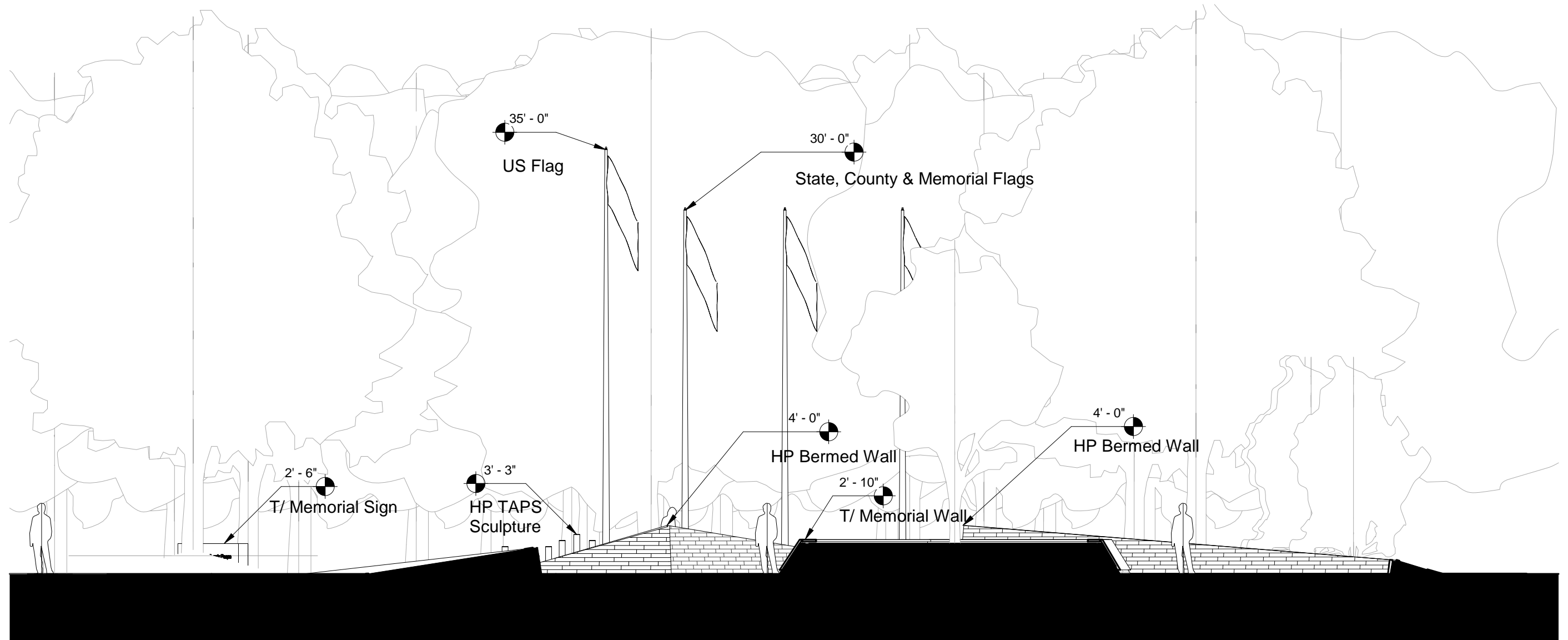
1 Plaza Section 1/8" = 1'-0"
