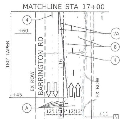
ROAD CONSTRUCTION AHEAD (W20-1103(O)-48) 350' 10'-6" (W12-1102(O)-48) ILLINOIS 58 (M1-1100-2424, M6-1(O)-2115) 350' WORK ZONE SPEED LIMIT 40 PHOTO ENFORCED $250 FINE MINIMUM (W21-1115(O)-3618, R2-1-3648, R10-1108p-3618, R2-1106p-3618) 150' END WORK ZONE SPEED LIMIT (G20-1103-6036) PLACED ON NORTHBOUND SIDE OPPOSITE WZSL ASSEMBLY W21-1(O)-48* (W21-1(O)-48*) 350' * MUST BE REMOVED OR COVERED WHEN WORKERS ARE NOT PRESENT FOR MORE THAN ONE HOUR.
